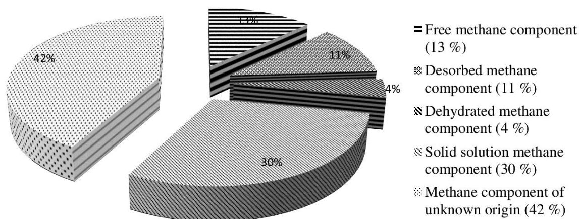
Figure 2 – Possible content of methane phase components in its total average volume ( \approx 200 \text{ m}^3/\text{t} ) during GDP
